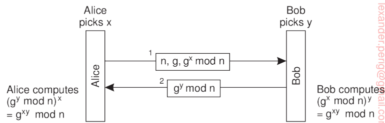
Figure 9.26: The principle of Diffie-Hellman key exchange.
